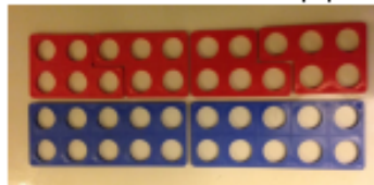
4 groups of 5 are equal to 20
